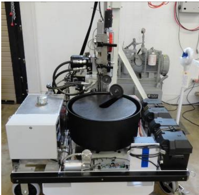
ZGS-10000-6-1 Mobile Hydraulic RHGSE (shown with MagSens Head already installed)
